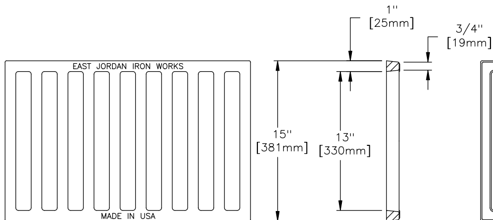
SECTION OF GRATE
