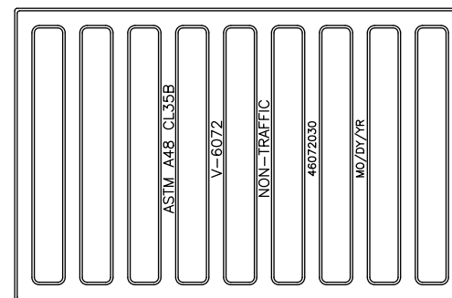
BACKSIDE OF GRATE
