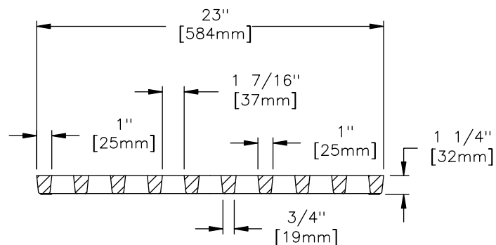
SECTION OF GRATE
